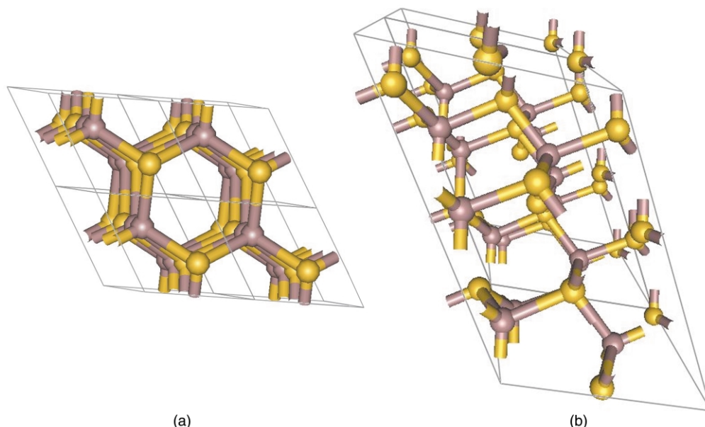
Fig. 1 Structures of GaS (a) and \alpha\text{-Ga}_2\text{S}_3 (b).
