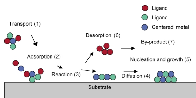
Fig. 5 Schematic diagram of the CVD process.
