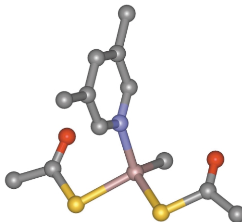
Fig. 11 Crystal structure of [GaMe(SCOMe) 2 (dmpy)].
